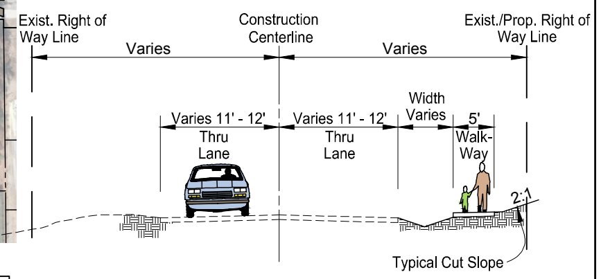
196TH ST SE TYPICAL ROADWAY CROSS SECTION NTS
