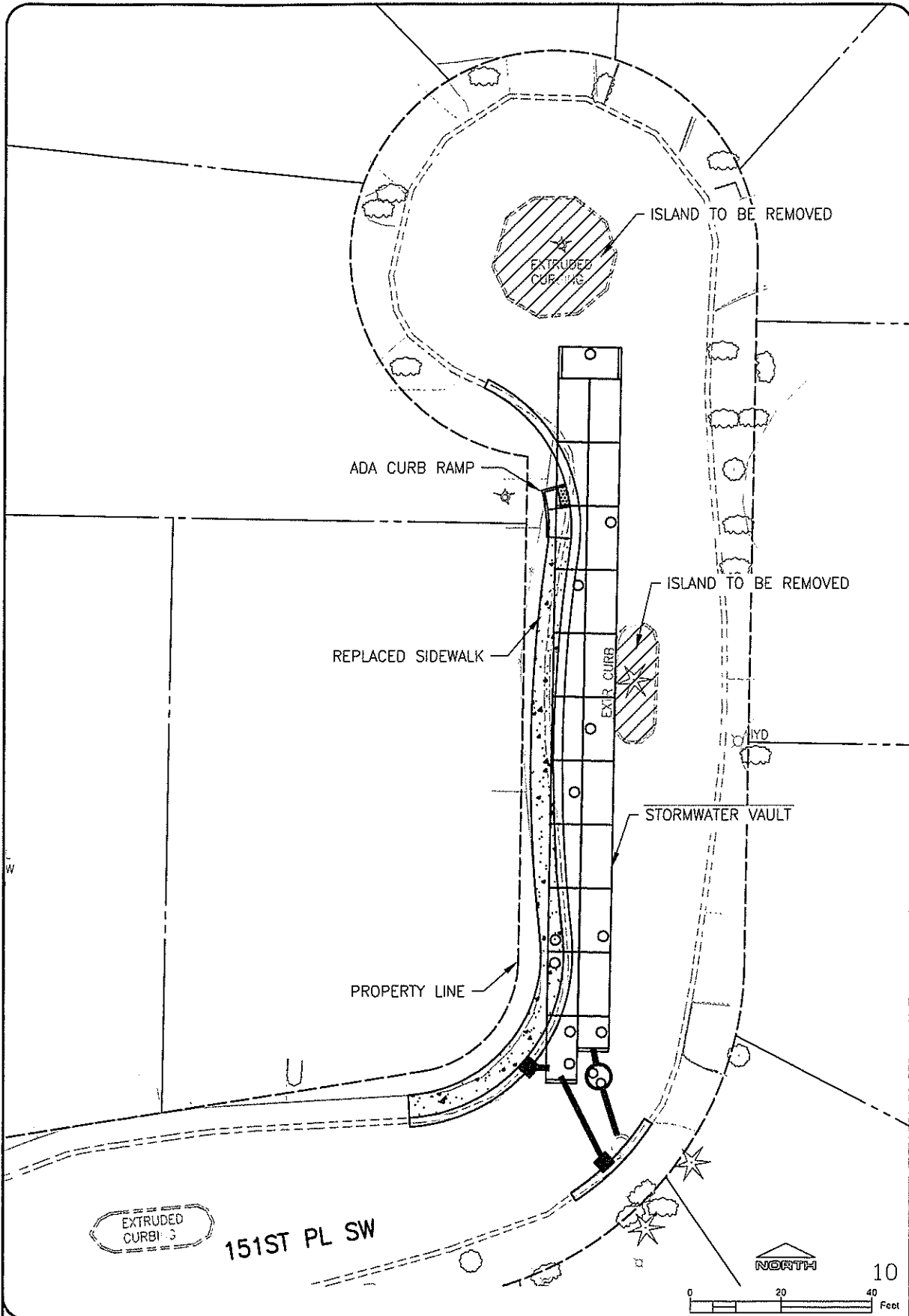
Stormwater Facility Retrofit near 5516 151st Pl SW (Hemlock Acres)
