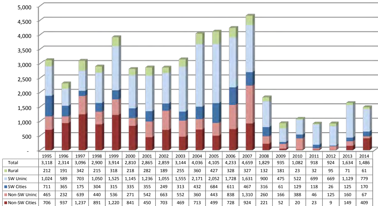
Figure RD-1 New Residential Lots in Recorded Formal Plats & Segregated-Lot Condos Lots Recorded By Year and General Area
