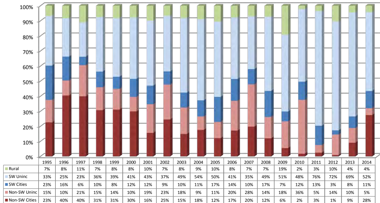
Figure RD-2 New Residential Lots in Recorded Formal Plats & Segregated-Lot Condos Percent of Lots Recorded by Year and General Area
